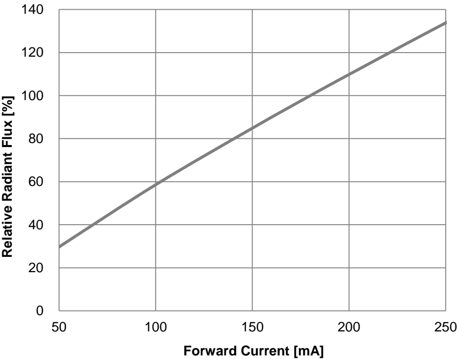
Fig 3. Forward Current vs. Relative Radiant Flux, T s =25°C
