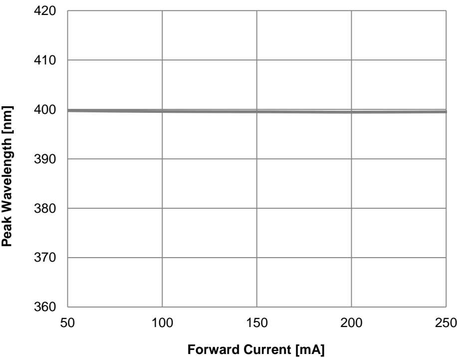
Fig 4. Forward Current vs. Peak Wavelength, T s =25°C
