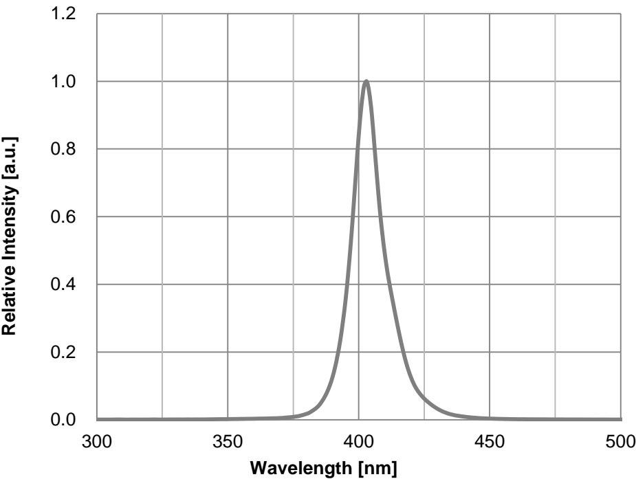
Fig 1. Spectrum, T_s=25^{\circ}\text{C} , I_F=180\text{mA}
