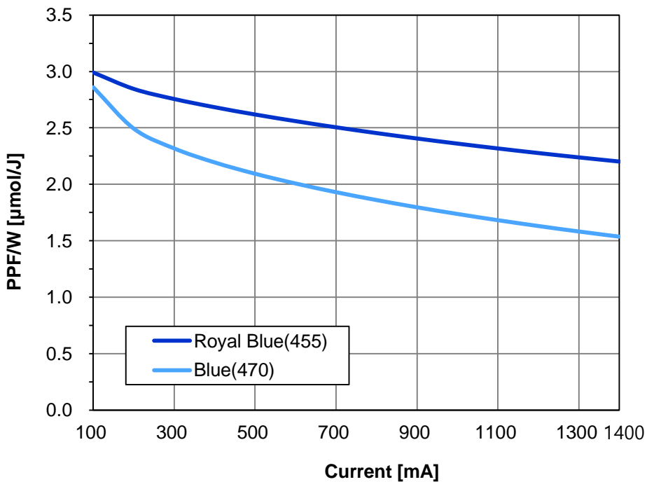
Fig 10-1. Current vs \mu\text{mol/s} characteristics
