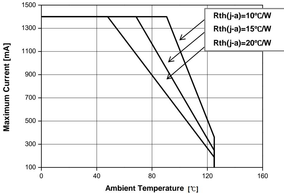
Fig 9. Maximum Forward Current vs. Ambient Temperature, T_j(\text{max.})=135^\circ\text{C}
