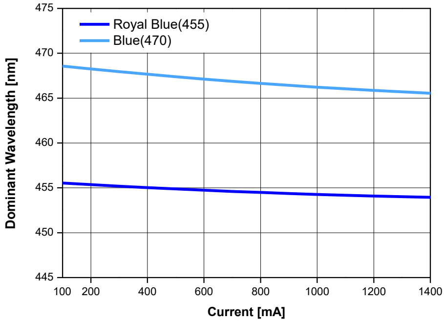
Fig 5. Forward Current vs. Dominant Wavelength, T_a=25^{\circ}\text{C}
