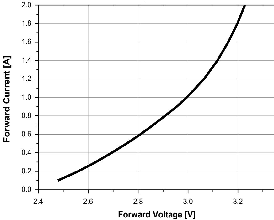
Forward Voltage vs. Forward Current, T_j=85^\circ\text{C}
