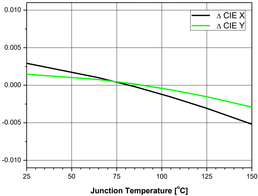
Fig 6. Junction Temp. vs. CIE X, Y Shift, I_F=1050\text{mA}
