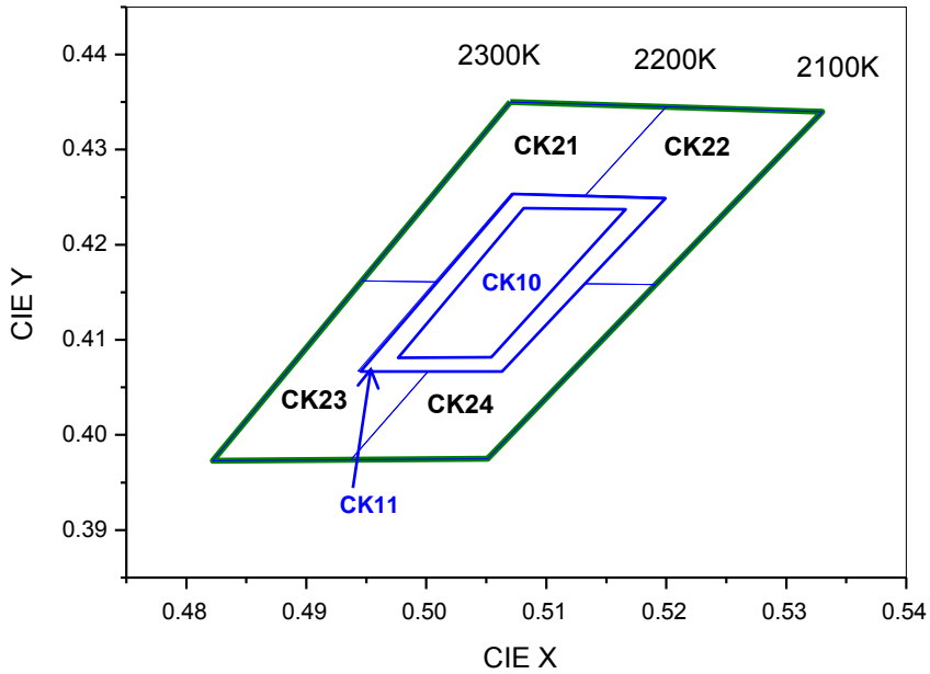
CIE Chromaticity Diagram T_j=25^\circ\text{C} , I_F=150\text{mA}
