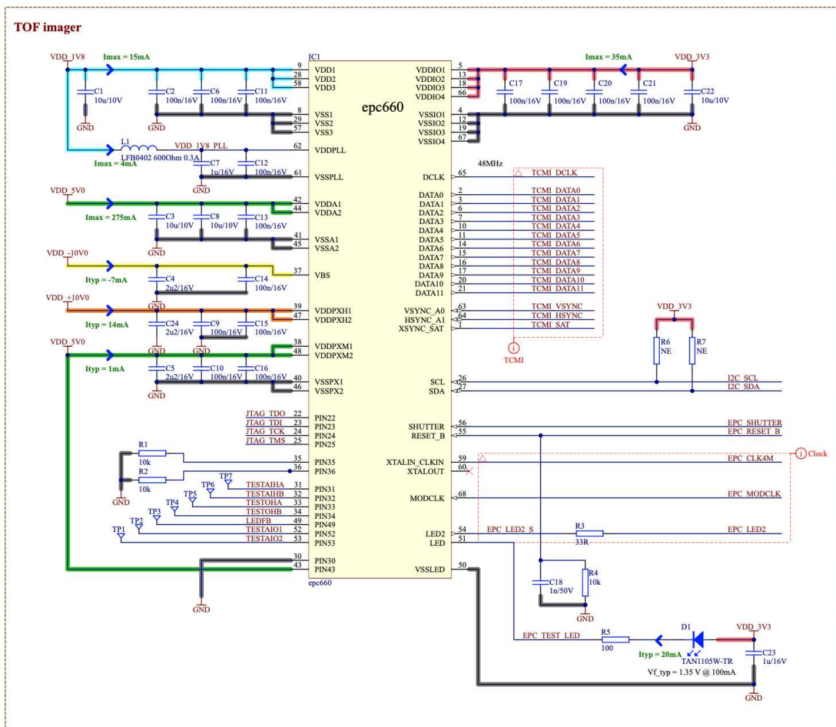
Figure 2: Schematic diagram - TOF imager
