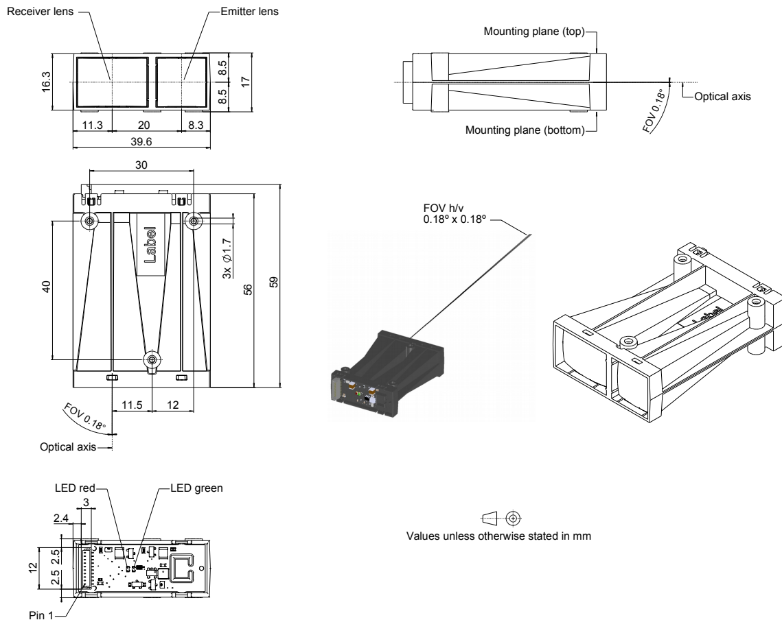
Figure 3: Mechanical dimensions
